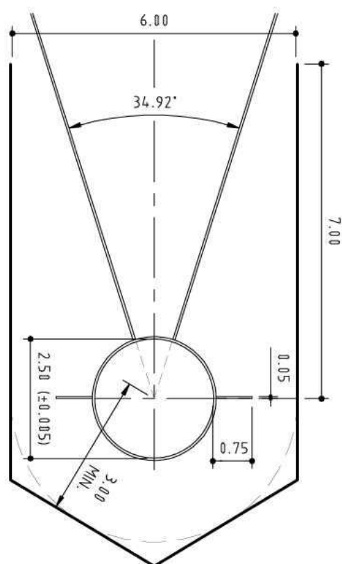
Figur TR 35 – Bur for diskoskast
