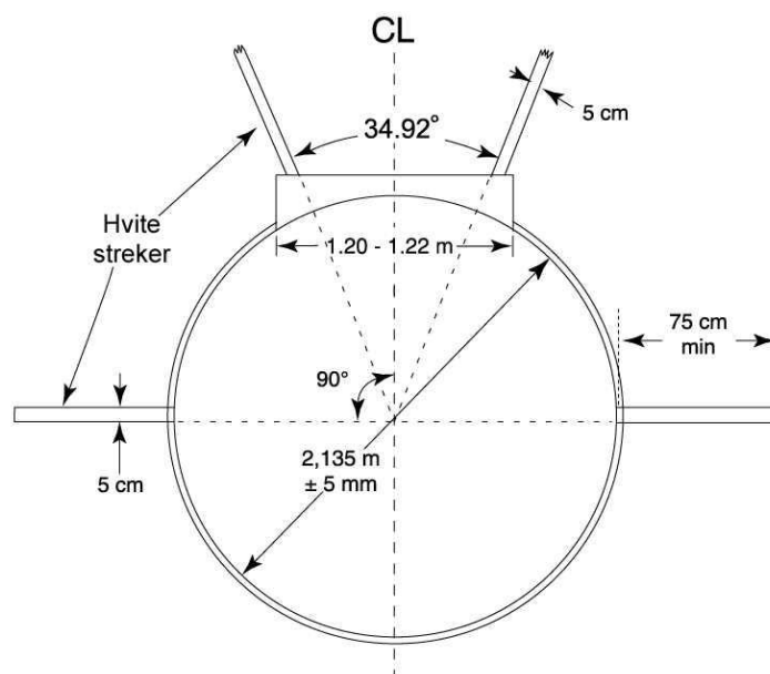
Figur (a) TR 32 – kuling
