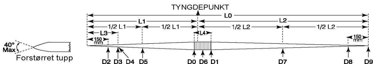
Figur TR 38 – spyd
