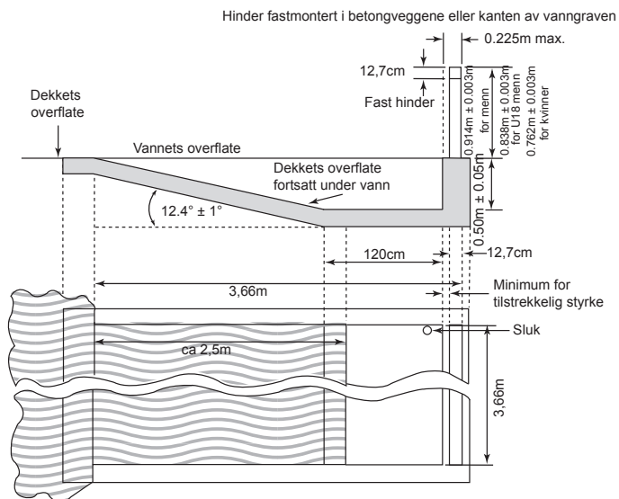
Figur (b) TR 23 - Vanngrav
