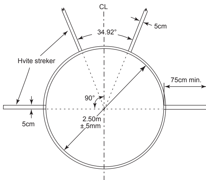
Figur (b) TR 32 - diskosring
