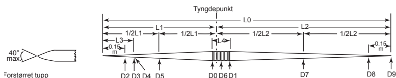
Figur TR 38 – spyd
